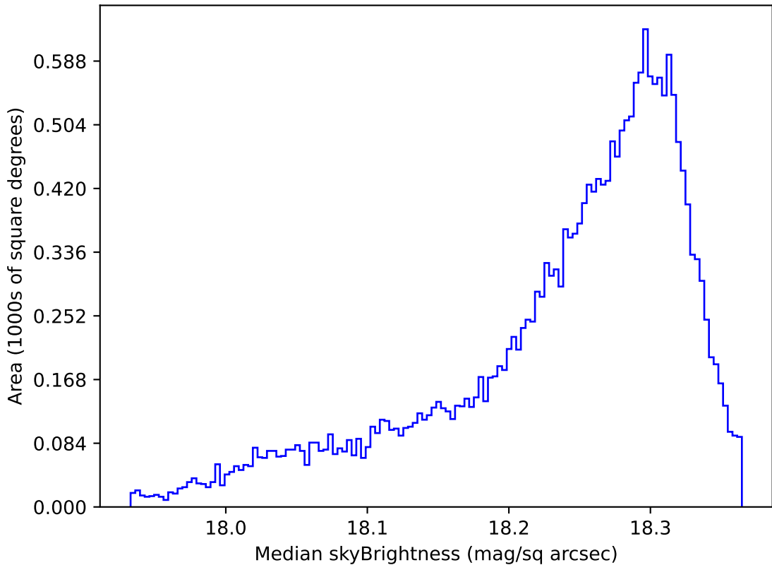
weather_cloudso18v3.4_10yrs All sky y band: Median skyBrightness
