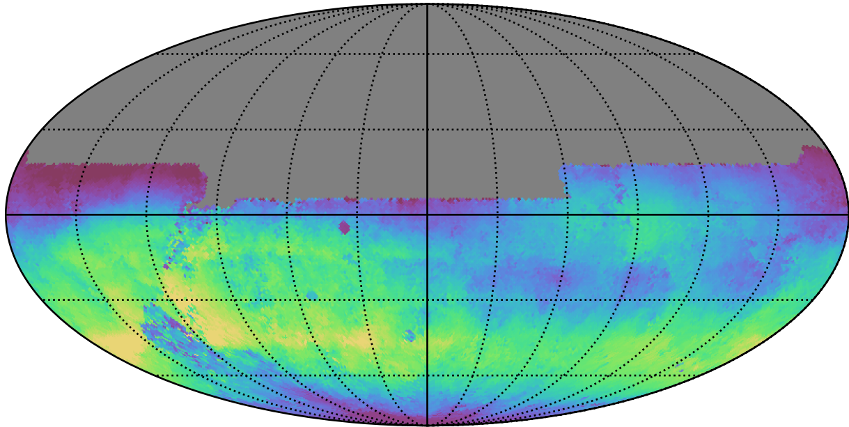
weather_cloudso18v3.4_10yrs All sky u band: Median skyBrightness
