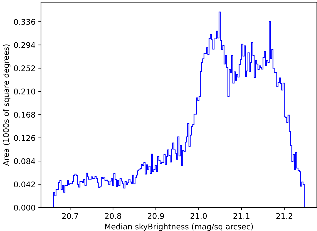
weather_cloudso18v3.4_10yrs All sky r band: Median skyBrightness
