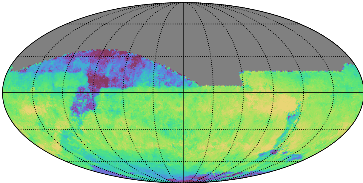
weather_cloudso18v3.4_10yrs All sky i band: Median skyBrightness
