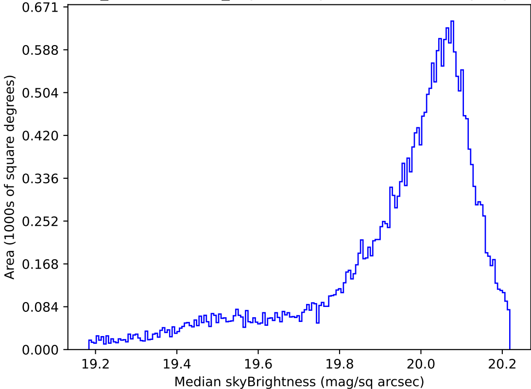
weather_cloudso18v3.4_10yrs All sky i band: Median skyBrightness
