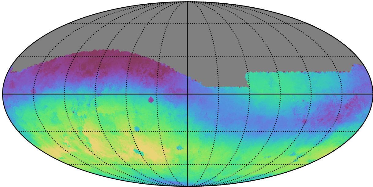
weather_cloudso18v3.4_10yrs All sky g band: Median skyBrightness
