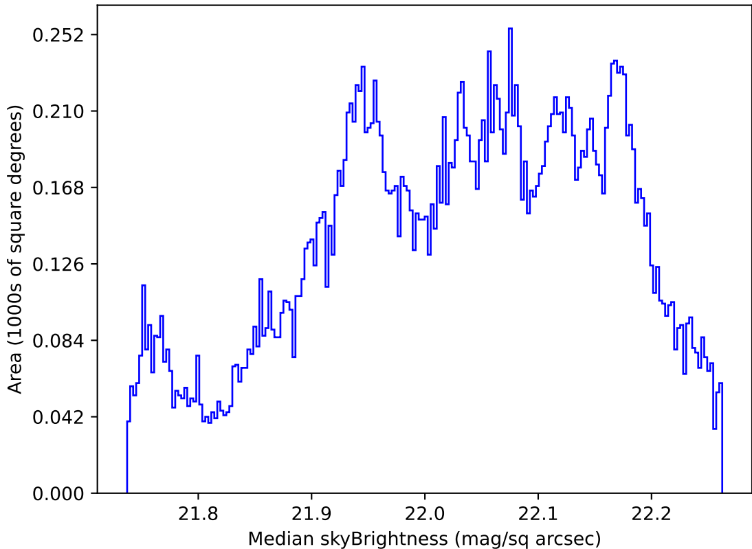
weather_cloudso18v3.4_10yrs All sky g band: Median skyBrightness
