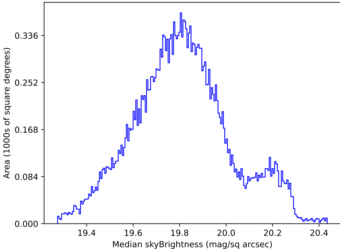
weather_cloudso18v3.4_10yrs All sky all bands: Median skyBrightness
