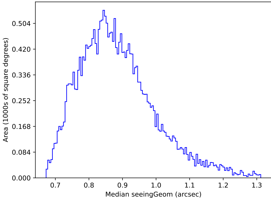
weather_cloudso18v3.4_10yrs Yr 1 z band: Median seeingGeom
