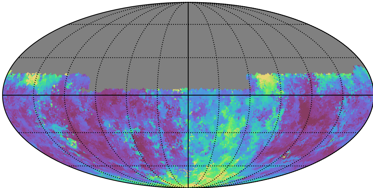
weather_cloudso18v3.4_10yrs Yr 1 u band: Median seeingGeom
