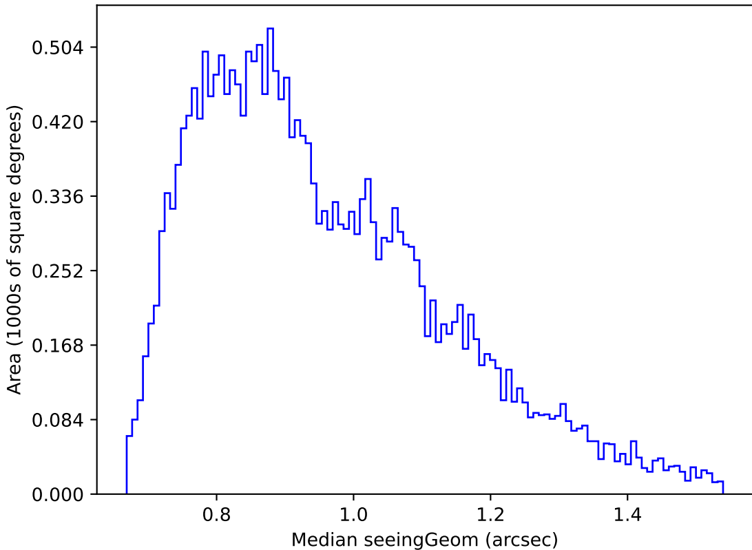
weather_cloudso18v3.4_10yrs Yr 1 u band: Median seeingGeom
