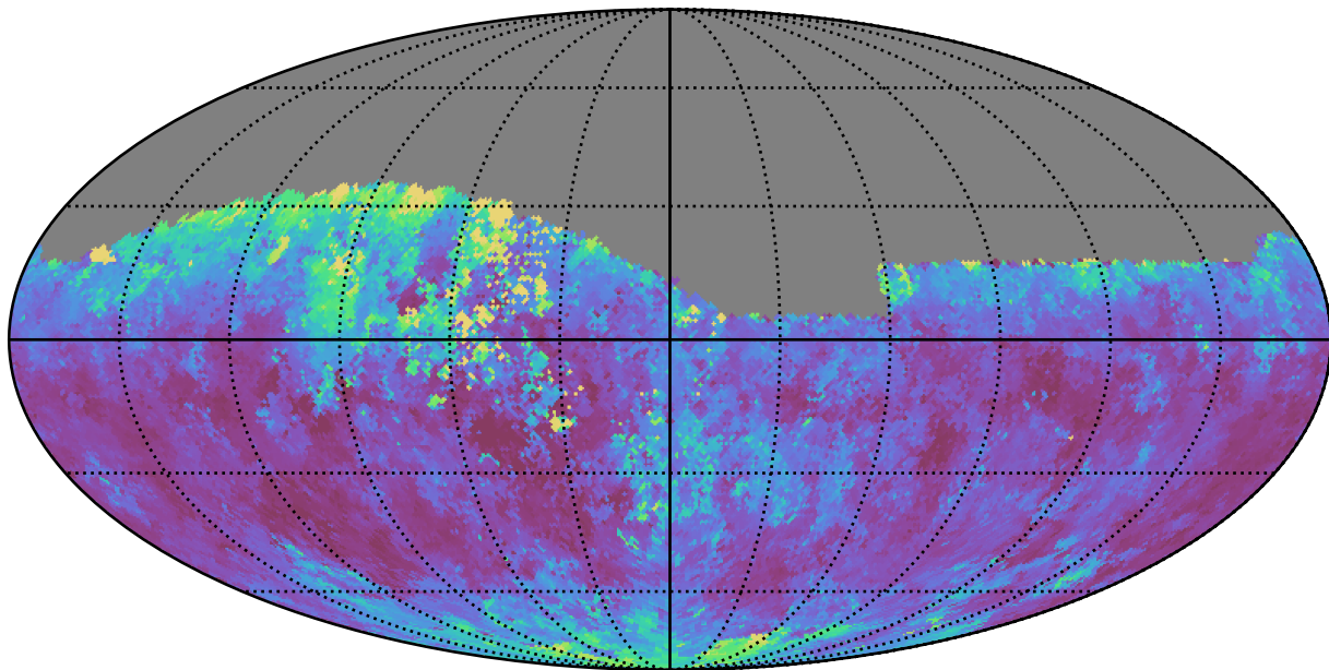
weather_cloudso18v3.4_10yrs Yr 1 i band: Median seeingGeom
