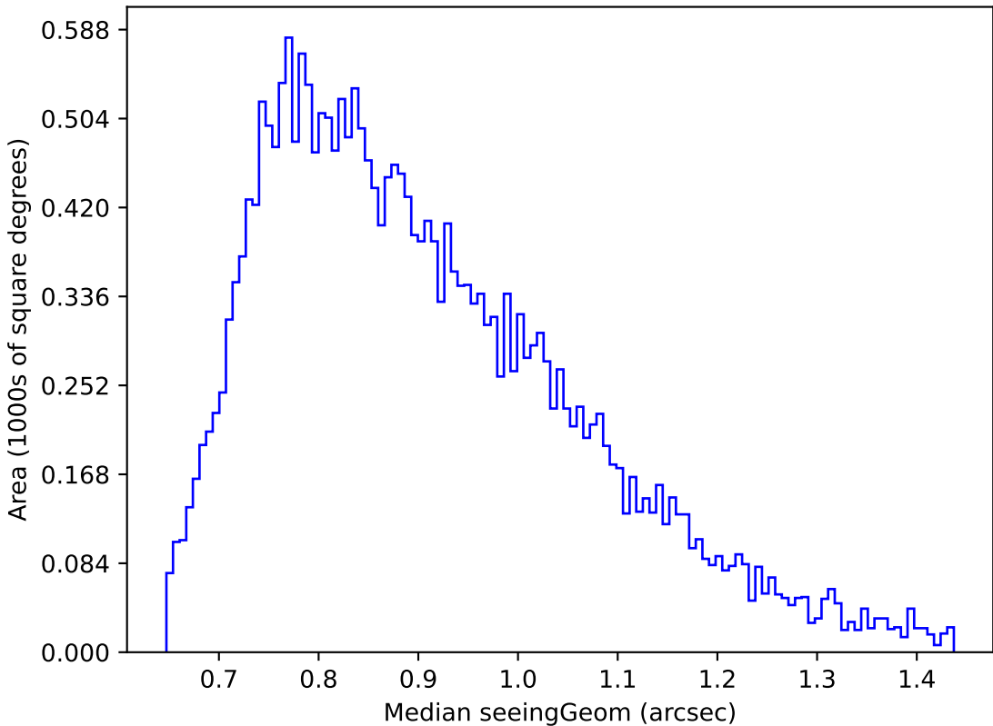
weather_cloudso18v3.4_10yrs Yr 1 g band: Median seeingGeom
