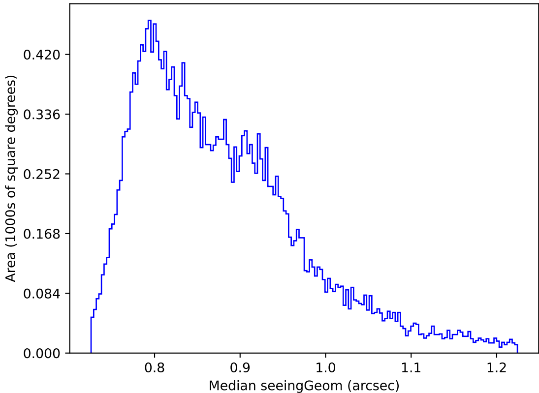
weather_cloudso18v3.4_10yrs Yr 1 all bands: Median seeingGeom
