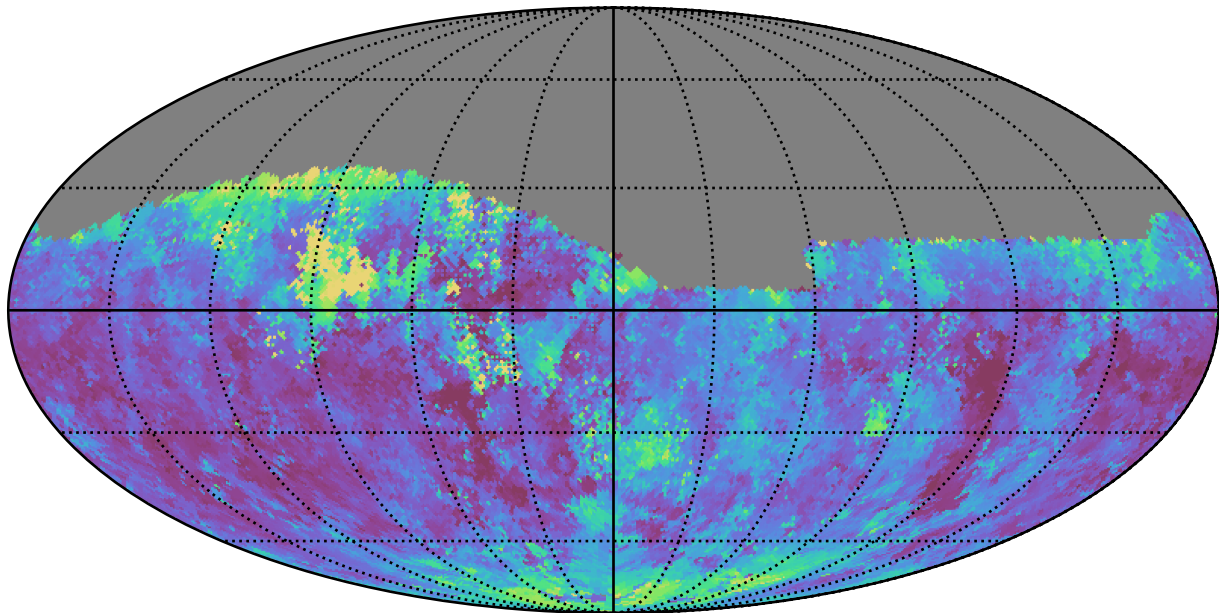
weather_cloudso18v3.4_10yrs Yr 1 z band: Median seeingEff
