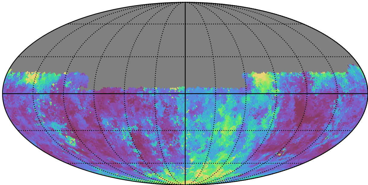
weather_cloudso18v3.4_10yrs Yr 1 u band: Median seeingEff
