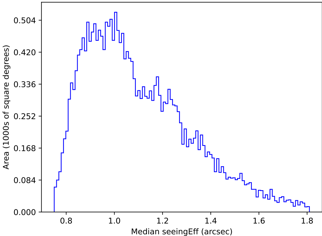
weather_cloudso18v3.4_10yrs Yr 1 u band: Median seeingEff
