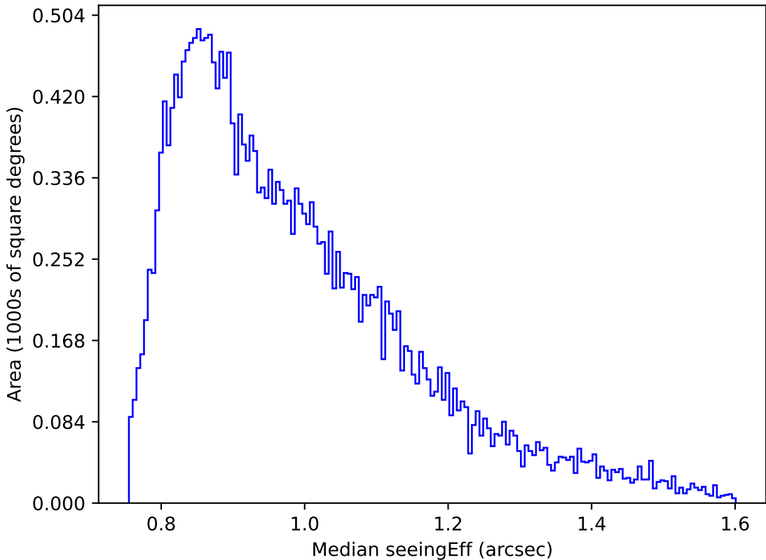
weather_cloudso18v3.4_10yrs Yr 1 r band: Median seeingEff
