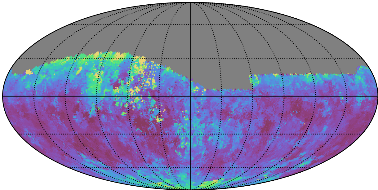
weather_cloudso18v3.4_10yrs Yr 1 i band: Median seeingEff
