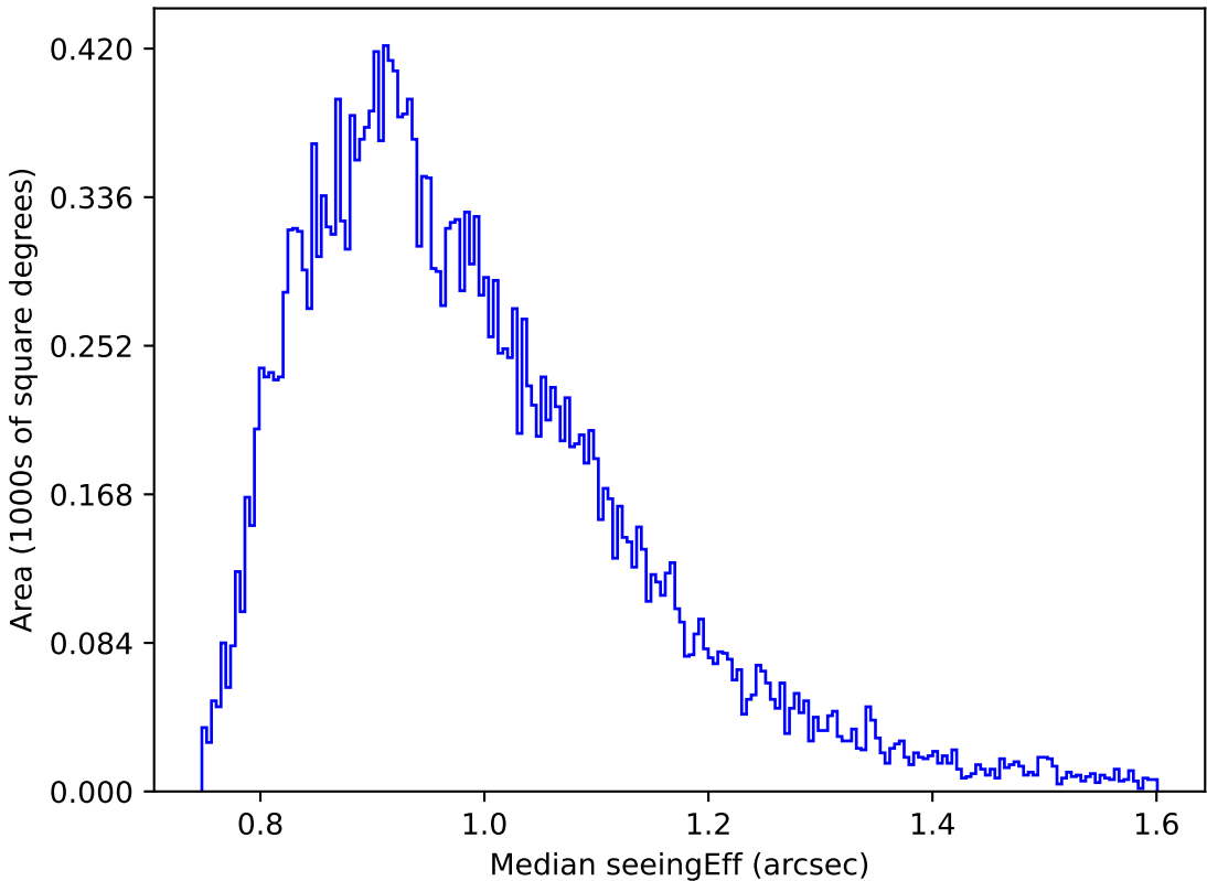
weather_cloudso18v3.4_10yrs Yr 1 i band: Median seeingEff
