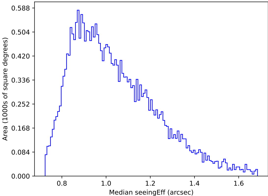
weather_cloudso18v3.4_10yrs Yr 1 g band: Median seeingEff
