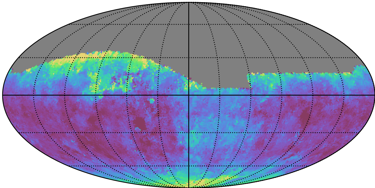
weather_cloudso18v3.4_10yrs Yr 1 all bands: Median seeingEff
