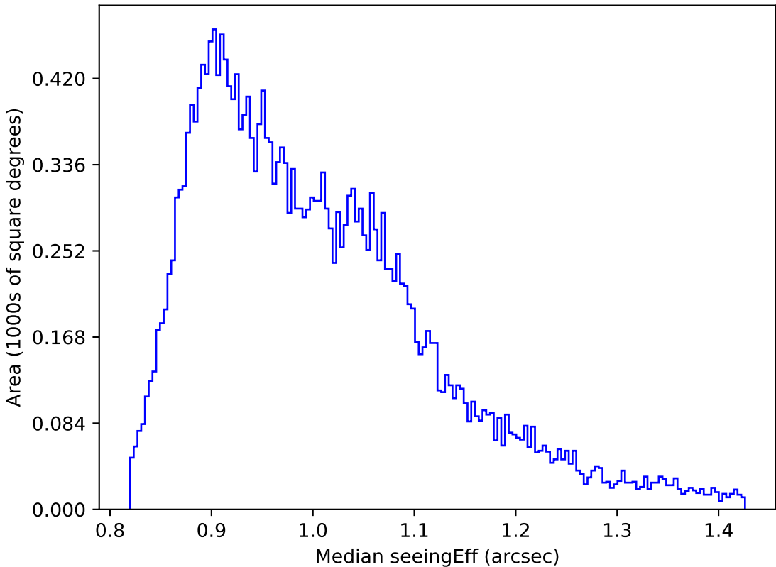
weather_cloudso18v3.4_10yrs Yr 1 all bands: Median seeingEff
