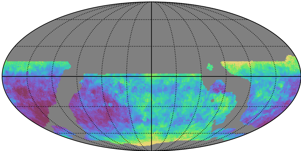
weather_cloudso18v3.4_10yrs WFD z band: Median seeingEff
