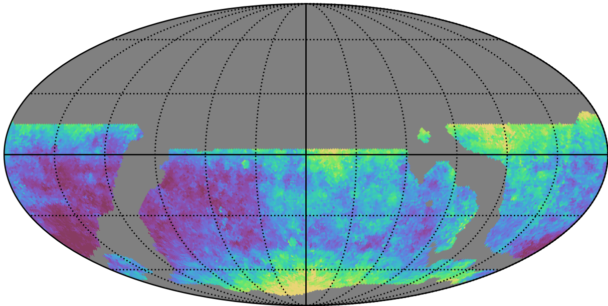
weather_cloudso18v3.4_10yrs WFD y band: Median seeingEff
