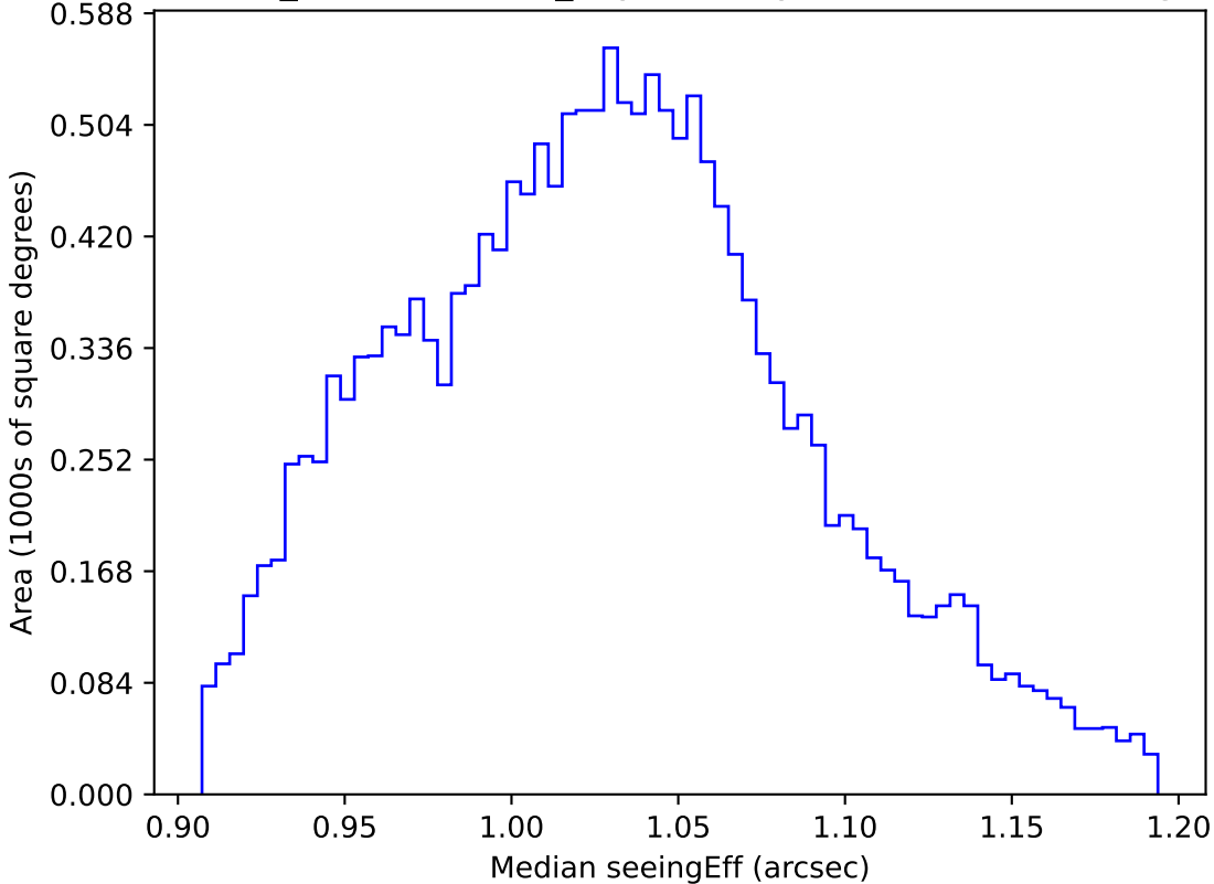
weather_cloudso18v3.4_10yrs WFD y band: Median seeingEff
