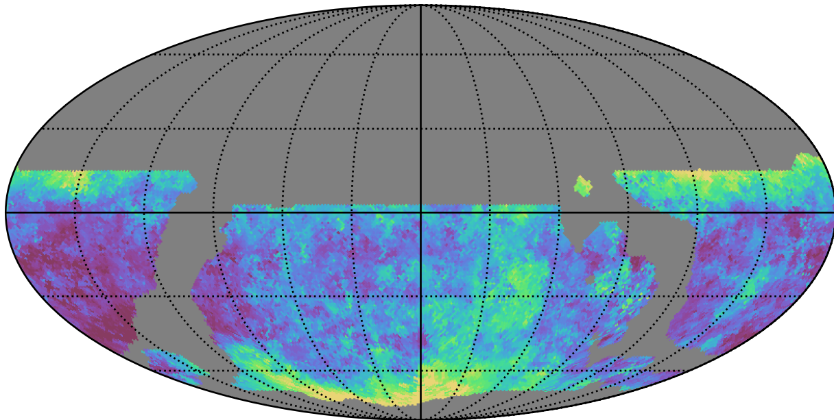
weather_cloudso18v3.4_10yrs WFD u band: Median seeingEff
