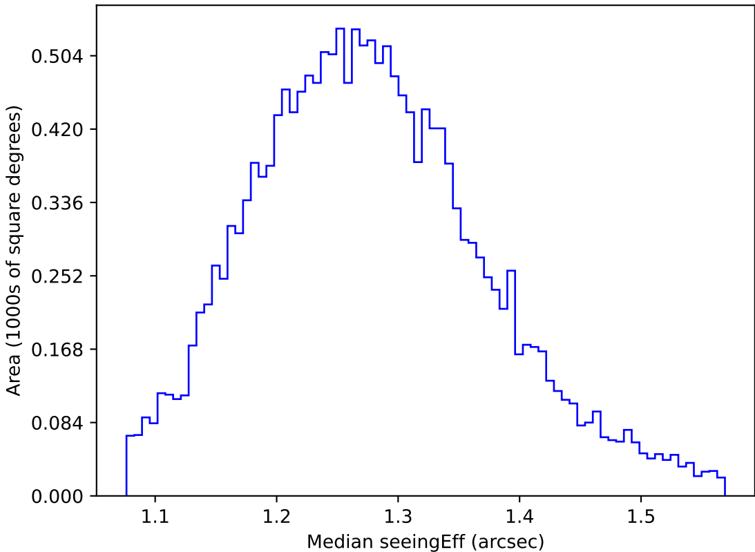
weather_cloudso18v3.4_10yrs WFD u band: Median seeingEff
