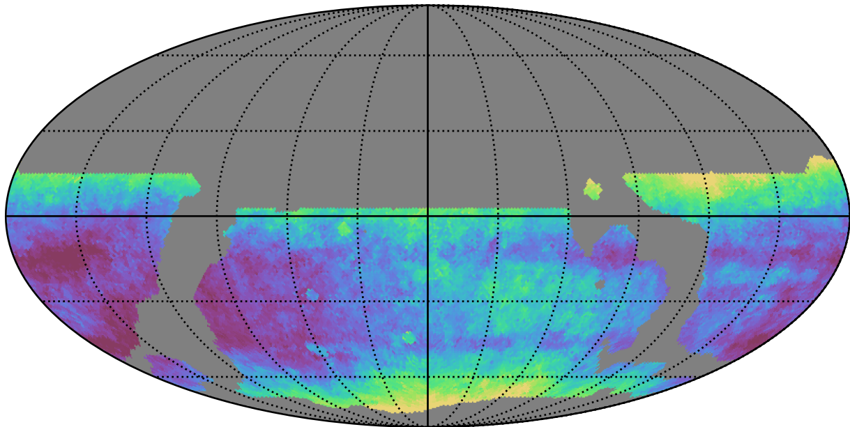
weather_cloudso18v3.4_10yrs WFD r band: Median seeingEff
