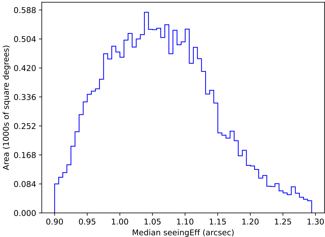
weather_cloudso18v3.4_10yrs WFD r band: Median seeingEff
