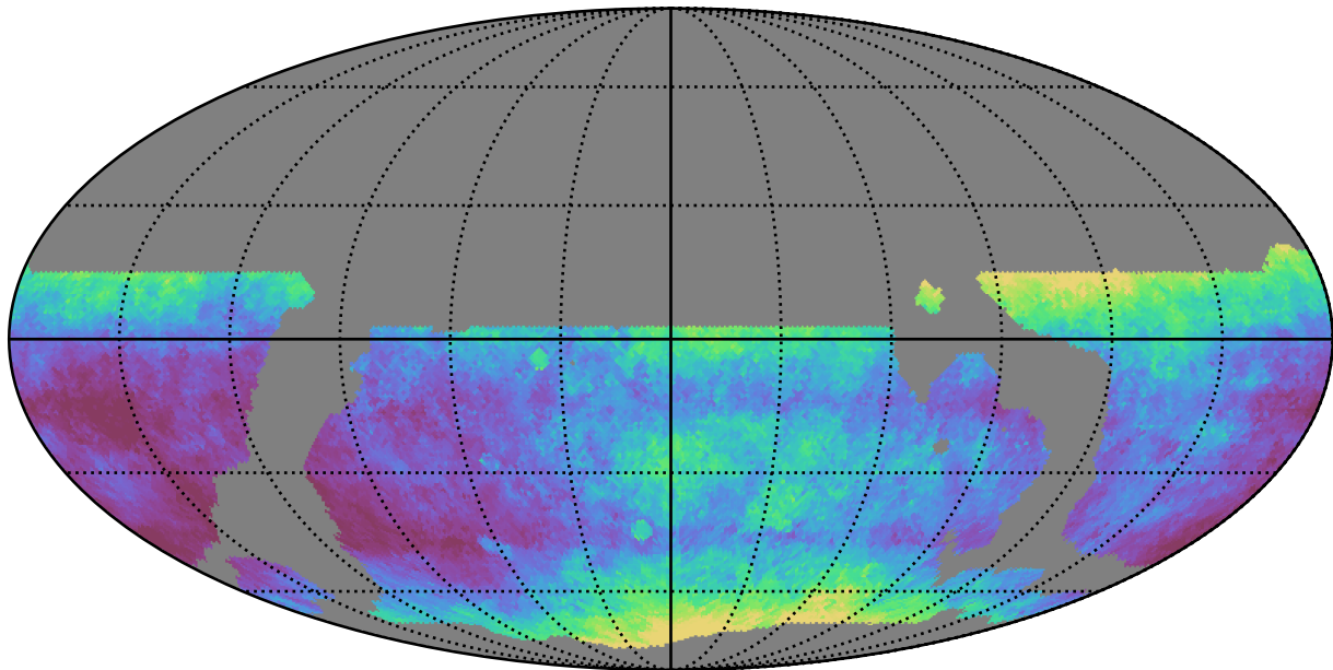
weather_cloudso18v3.4_10yrs WFD i band: Median seeingEff
