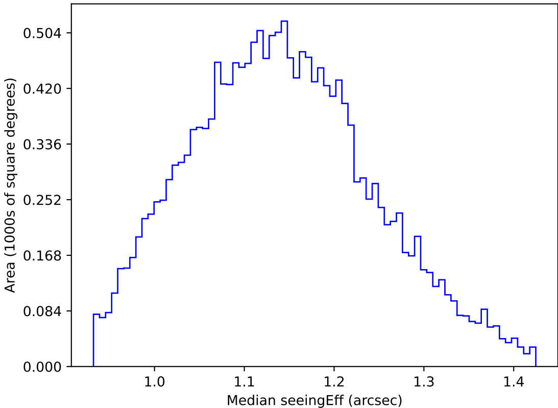
weather_cloudso18v3.4_10yrs WFD g band: Median seeingEff
