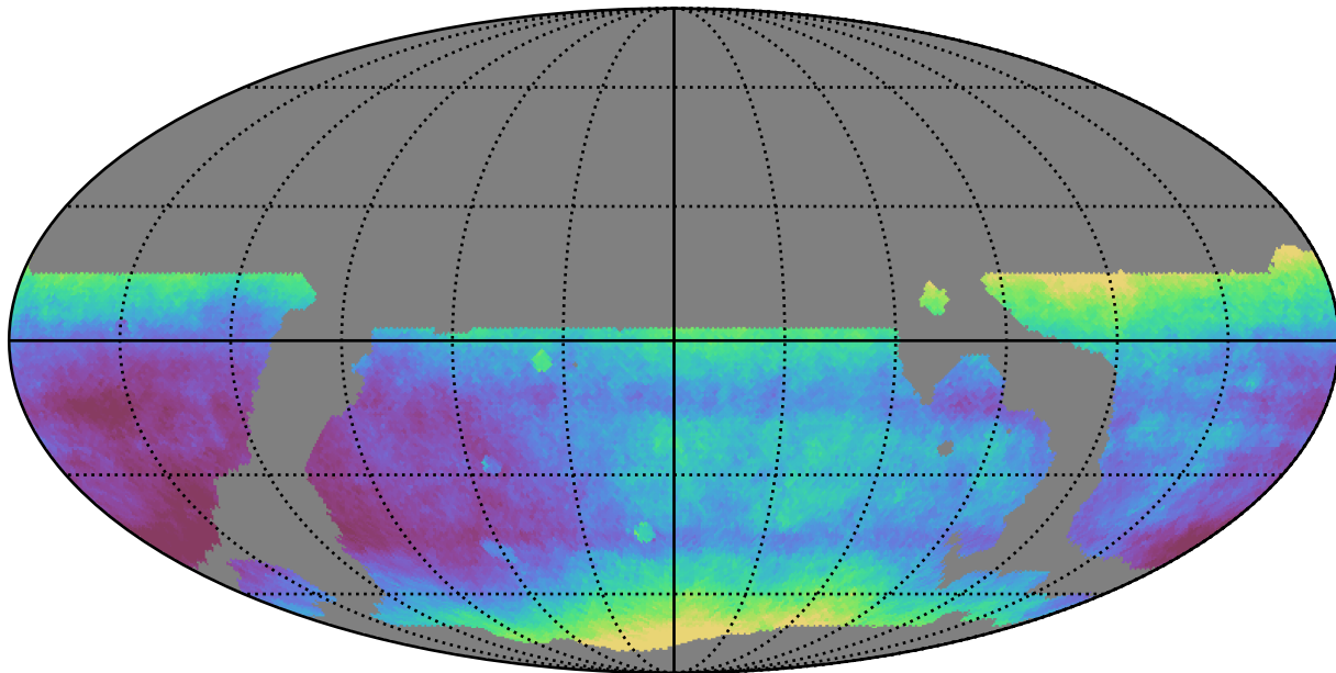
weather_cloudso18v3.4_10yrs WFD all bands: Median seeingEff
