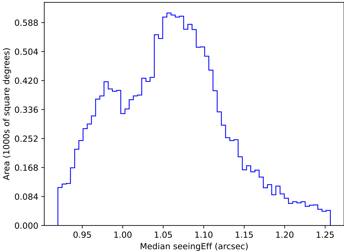
weather_cloudso18v3.4_10yrs WFD all bands: Median seeingEff
