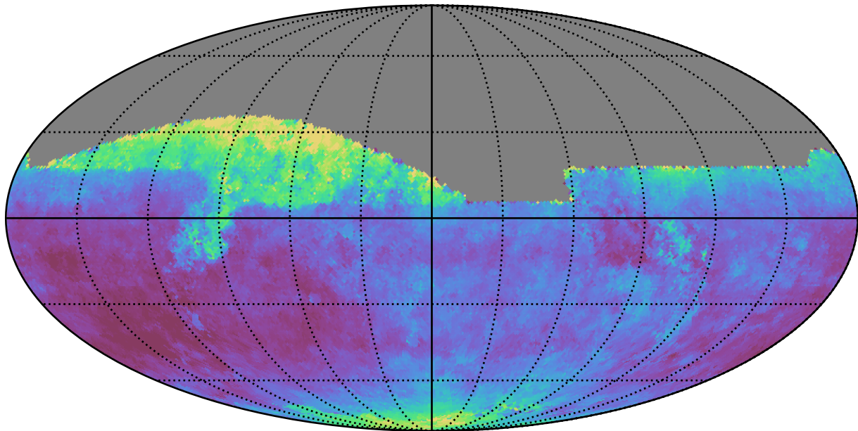
weather_cloudso18v3.4_10yrs All sky z band: Median seeingEff
