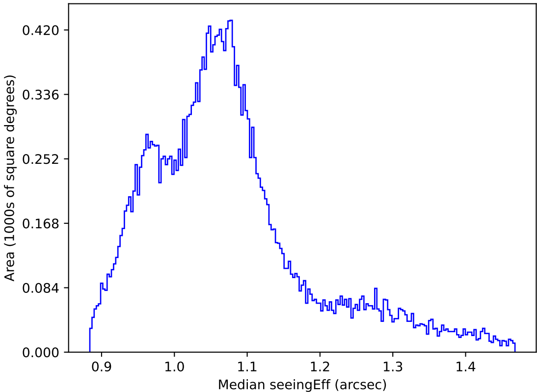
weather_cloudso18v3.4_10yrs All sky z band: Median seeingEff
