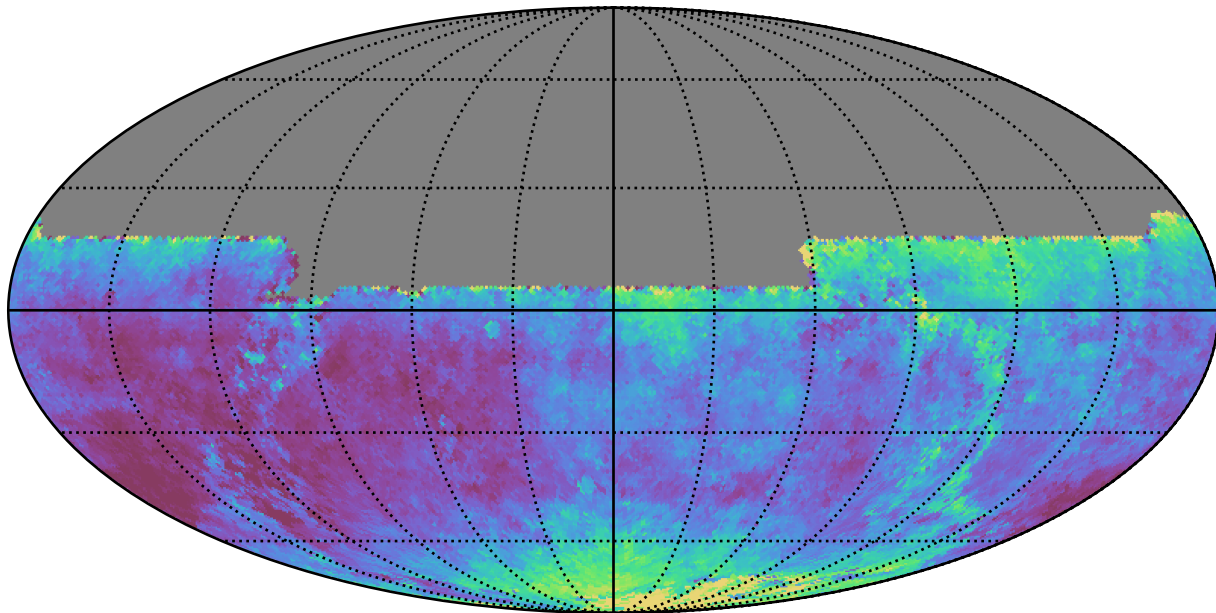
weather_cloudso18v3.4_10yrs All sky y band: Median seeingEff
