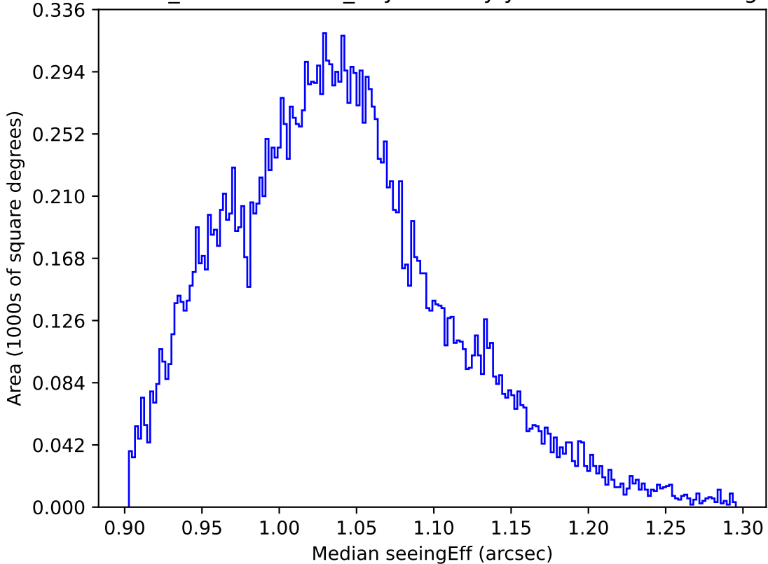
weather_cloudso18v3.4_10yrs All sky y band: Median seeingEff
