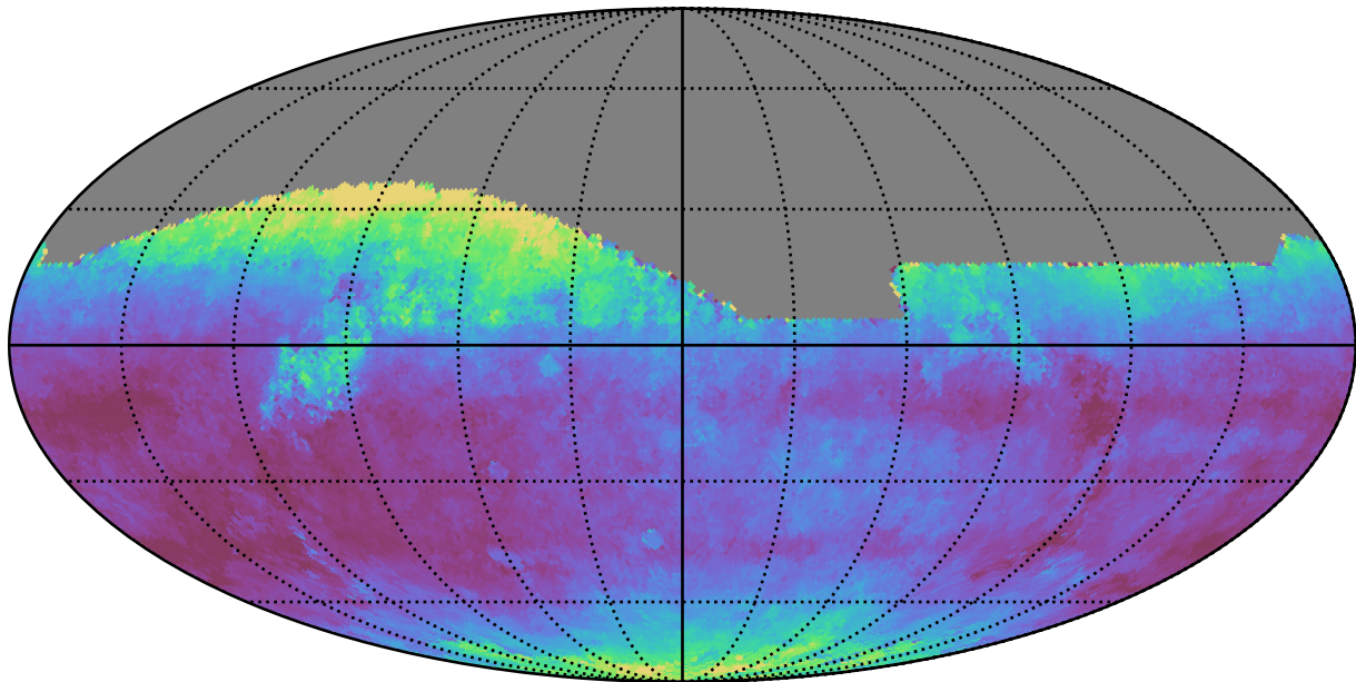
weather_cloudso18v3.4_10yrs All sky r band: Median seeingEff
