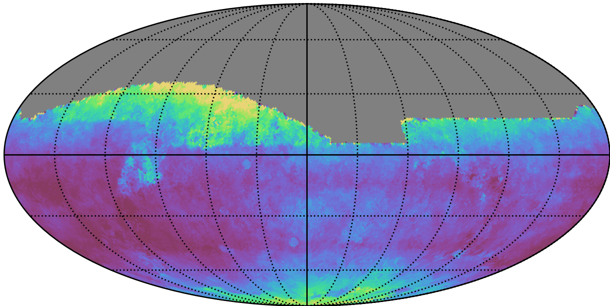
weather_cloudso18v3.4_10yrs All sky i band: Median seeingEff
