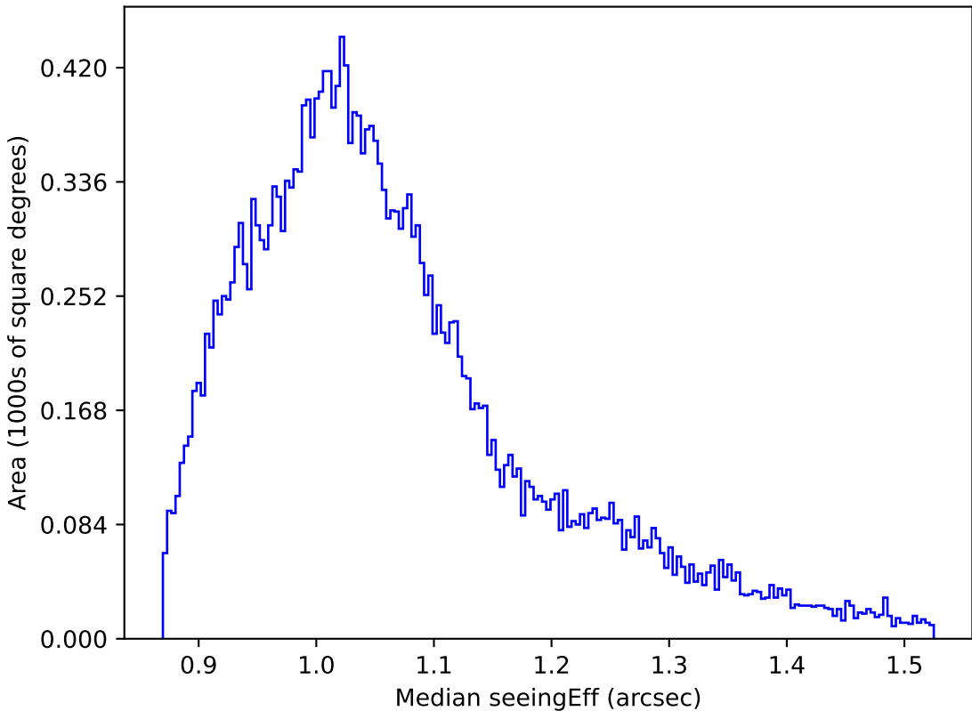
weather_cloudso18v3.4_10yrs All sky i band: Median seeingEff
