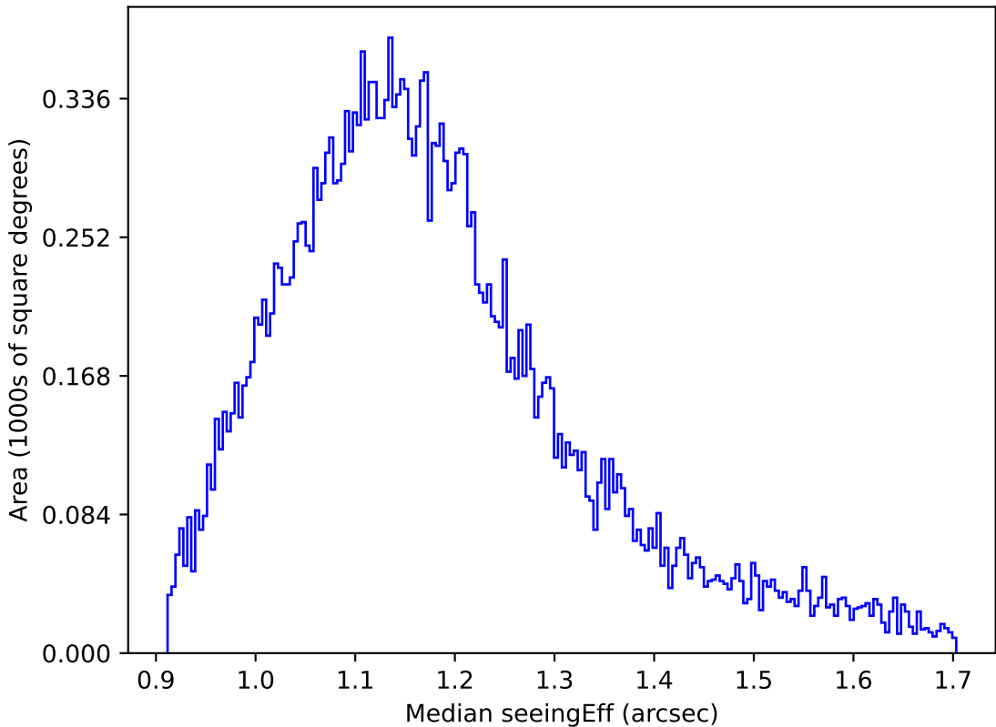
weather_cloudso18v3.4_10yrs All sky g band: Median seeingEff
