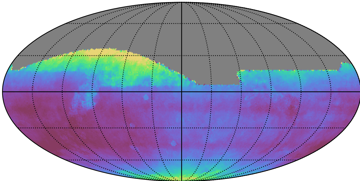
weather_cloudso18v3.4_10yrs All sky all bands: Median seeingEff
