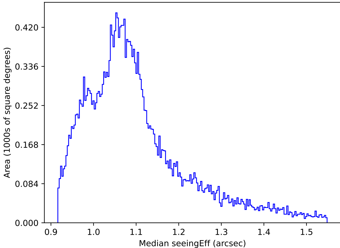
weather_cloudso18v3.4_10yrs All sky all bands: Median seeingEff
