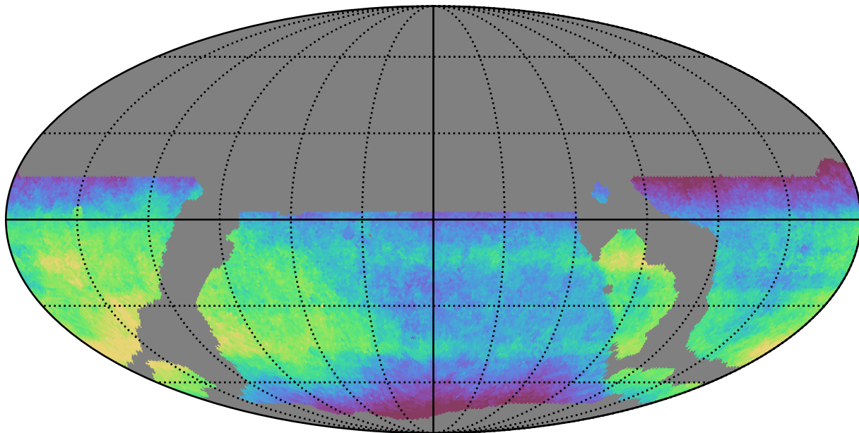
weather_cloudso18v3.4_10yrs WFD all bands: Median saturation_mag
