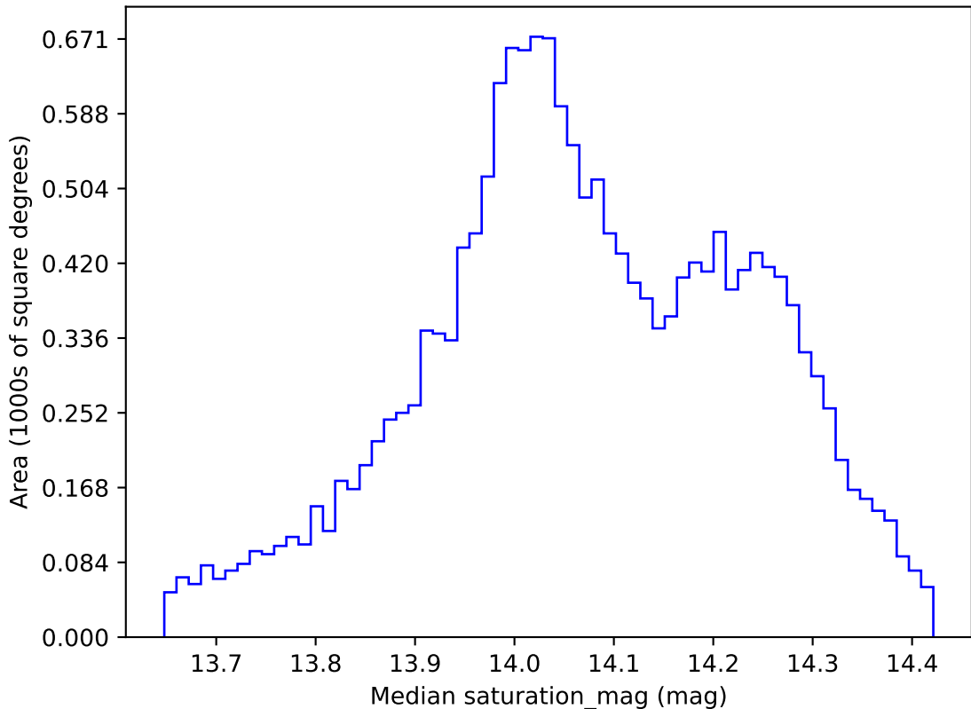
weather_cloudso18v3.4_10yrs WFD all bands: Median saturation_mag
