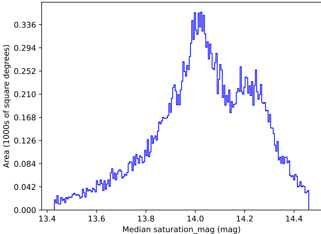
weather_cloudso18v3.4_10yrs All sky all bands: Median saturation_mag
