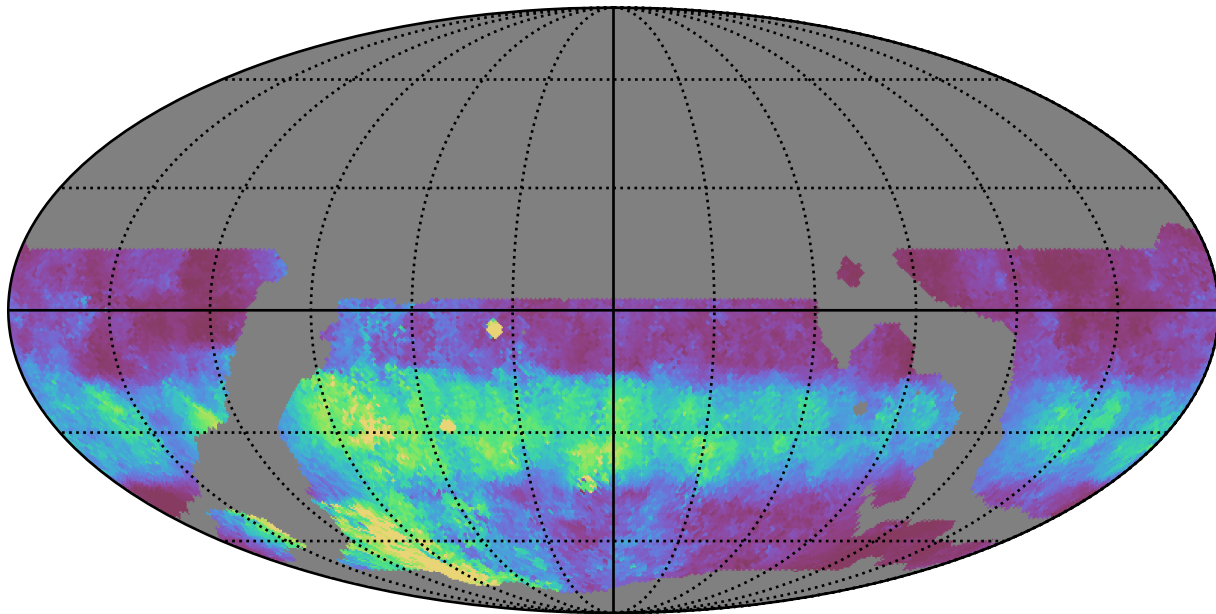
weather_cloudso18v3.4_10yrs WFD u band: Median normairmass
