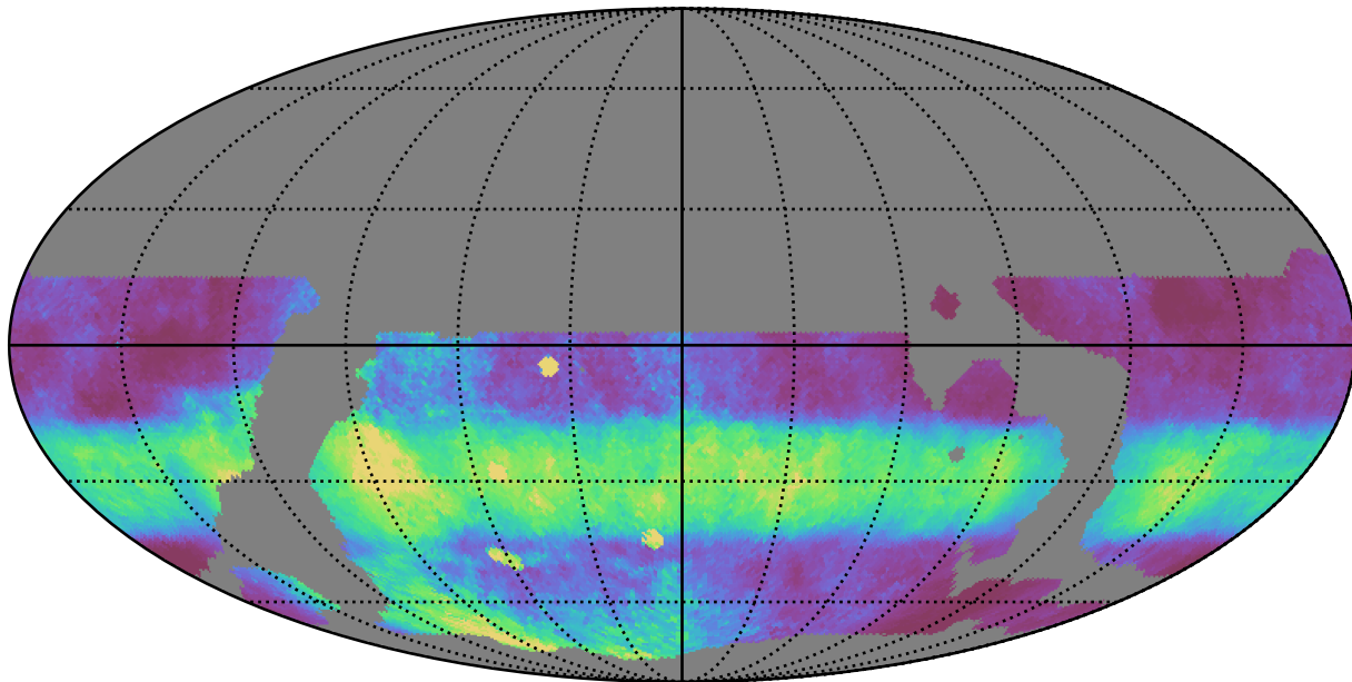
weather_cloudso18v3.4_10yrs WFD r band: Median normairmass
