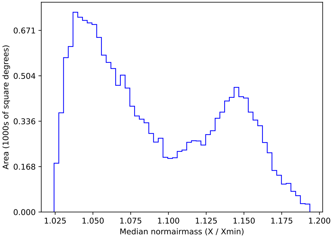
weather_cloudso18v3.4_10yrs WFD i band: Median normairmass
